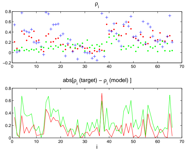
Figure 1: Model (green: hidden Gamma, red: Gamma Mix) Vs. empirical sector correlations (blue) & Errors.
